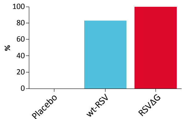
Figure 1. ITV-RSV-ΔG is highly immunogenic in cotton rats (A) and protects against challenge with wildtype RSV (B) after a single dose.
