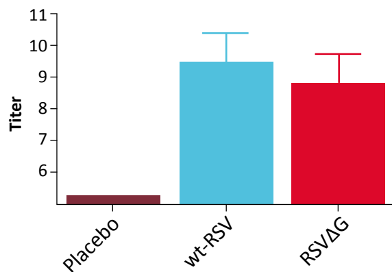
Figure 1. ITV-RSV-ΔG is highly immunogenic in cotton rats (A) and protects against challenge with wildtype RSV (B) after a single dose.
